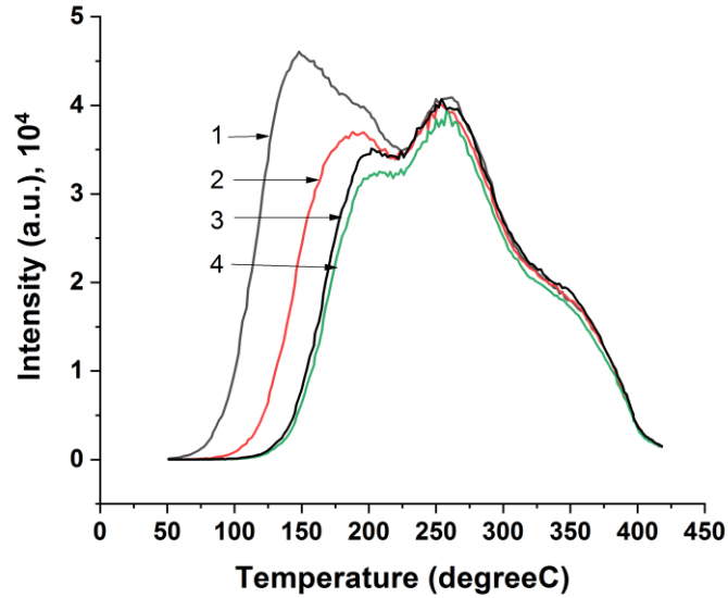
Fig. 2 TL glow curve of unheated natural feldspar irradiated at 34.12 Gy (1); TL glow curve of the same sample after 15 days (2); 22 days (3); and 27 days (4).
