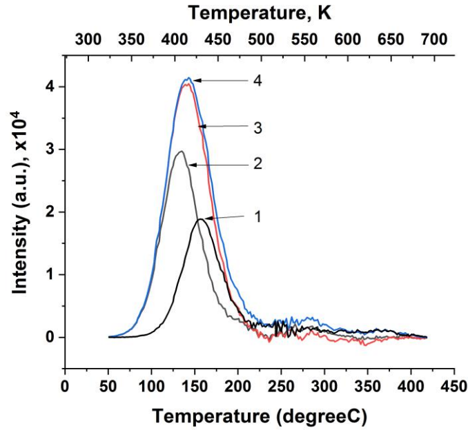
Fig. 4. Isolated glow curves obtained by subtracting method. Curve (1) represents the isolated peak by subtracting glow curve (4) presented in Fig.2 from curve (2) presented in Fig.2, i.e. (1) = Fig 2 curve (2) – Fig.2 curve (4); and subsequently (2) = Fig 2 curve (1) – Fig.2 curve (2); (3) = Fig 2 curve (1) – Fig.2 curve (3); (4) = Fig 2 curve (1) – Fig.2 curve (4)
