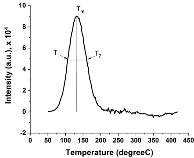
Fig. 1 Isolated TL peak. T_m is a temperature at the peak maximum; T_1 is a temperature at the point of left side half-width; T_2 is a temperature at the point of right side half-width.
