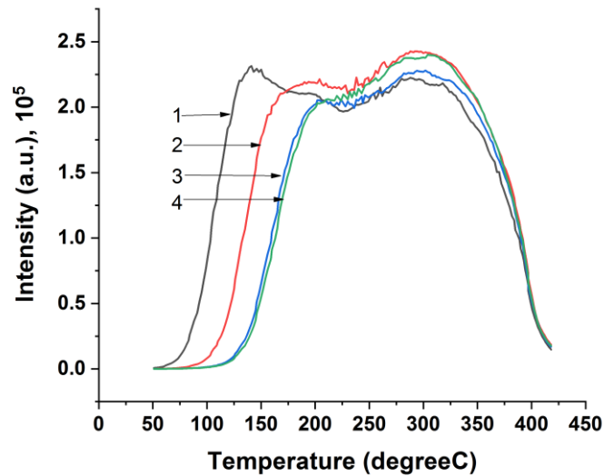
Fig. 3 TL glow curve of natural feldspar heated at 600°C for one hour and irradiated at 34.12 Gy (1); TL glow curve of the same sample after 5 days (2); 12 days (3); and 40 days (4). Curve (5) represents the isolated peak by subtracting curve (4) from curve (1)
