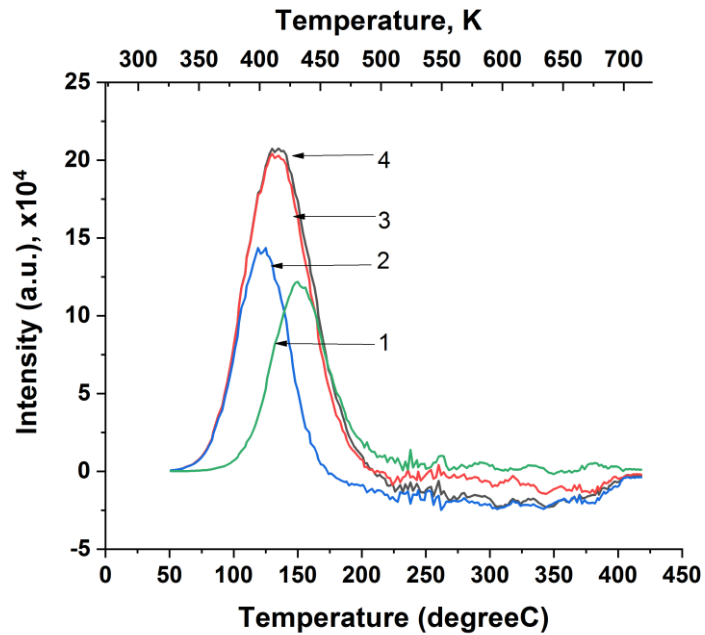
Fig. 5 Isolated glow curves obtained by subtracting method: Curve (1) represents the isolated peak by subtracting glow curve (4) presented in Fig.3 from curve (2) presented in Fig.3, i.e. (1) = Fig 3, curve (2) – Fig.3, curve (4); and subsequently (2)= Fig 3, curve (1) – Fig.3, curve (2); (3)= Fig 3, curve (1) – Fig.3, curve (3); (4) = Fig 3, curve (1) – Fig.3, curve (4)
