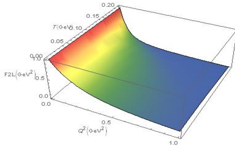
Fig. 3. The temperature dependence of excited F_{2L}(Q^2, T) left baryon form factor at n = 2 state.
