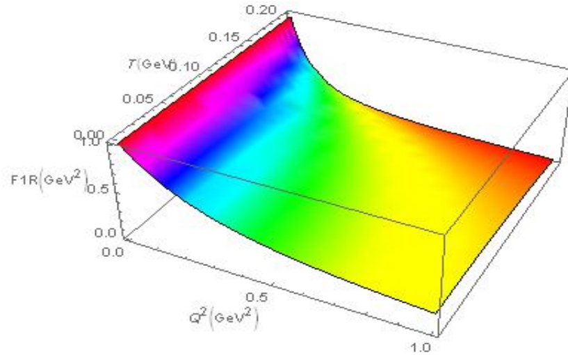
Fig. 2. The temperature dependence of excited F_{1R}(Q^2, T) right baryon form factor at n = 1 state.
