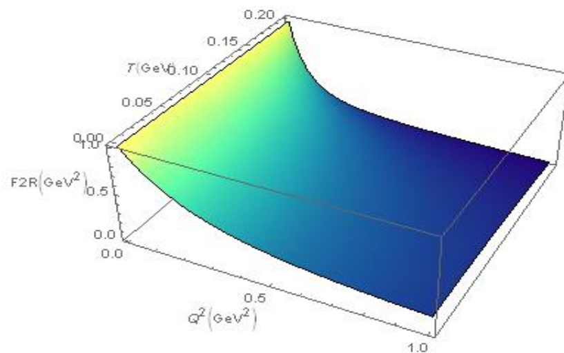
Fig. 4. The temperature dependence of excited F_{2R}(Q^2, T) right baryon form factor at n=2 state.
