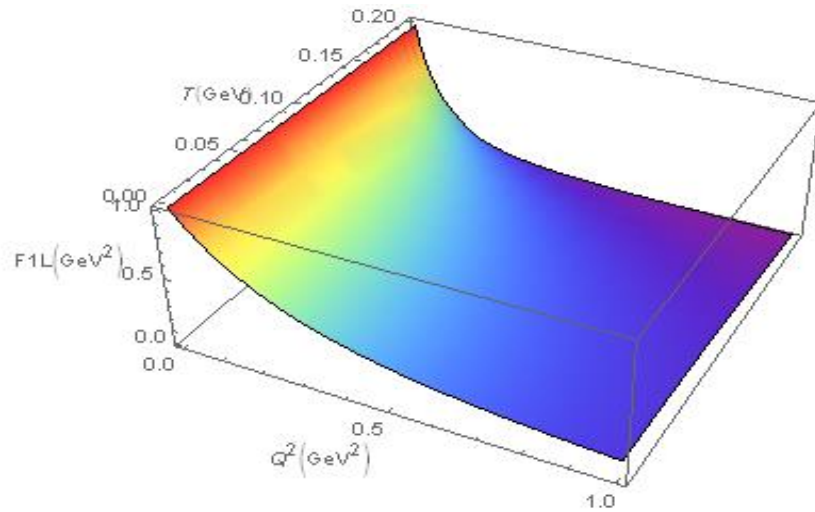
Fig. 1. The temperature dependence of excited F_{1L}(Q^2, T) left baryon form factor at n = 1 state.
