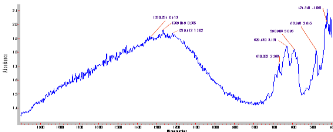
Fig. 1c. IR absorption spectrum of single crystal GaS after consequently 140 krad irradiation and annealing in vacuum ( 100^{\circ}\text{C} , 1 hour)
