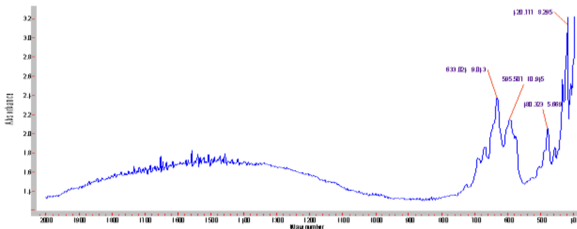
Fig. 1e. IR absorption spectrum of single crystal GaS after consequently 140 krad irradiation and annealing in vacuum (100 °C, 1 hour), open air (100 °C, 1 hour), open air (130 °C, 1 hour) and open air (150 °C, 1 hour)
