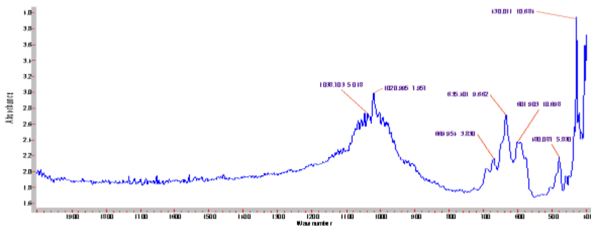
Fig 1d. IR absorption spectrum of single crystal GaS after consequently 140 krad irradiation and annealing in vacuum ( 100^{\circ}\text{C} , 1 hour) and open air ( 100^{\circ}\text{C} , 1 hour)
